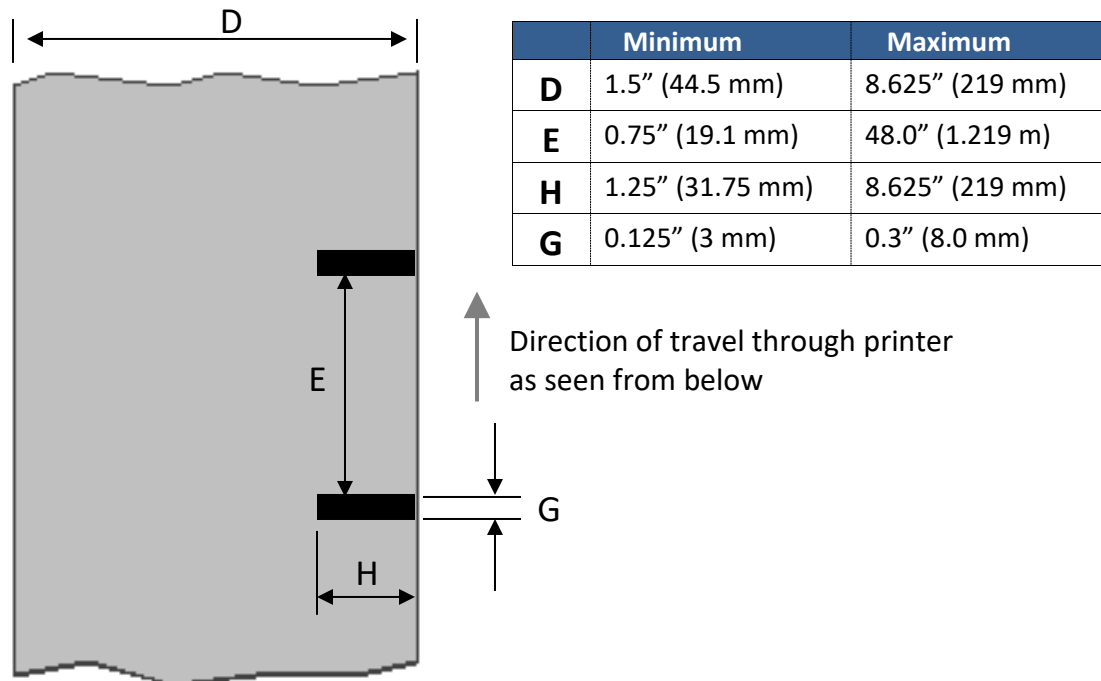
Figure 3: Black Mark (Reflective) Media
