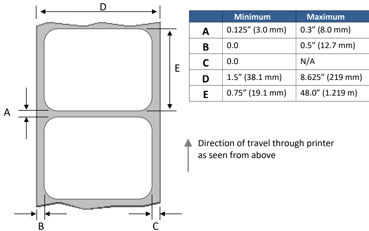
Figure 2: Gap (Transmissive) Media
