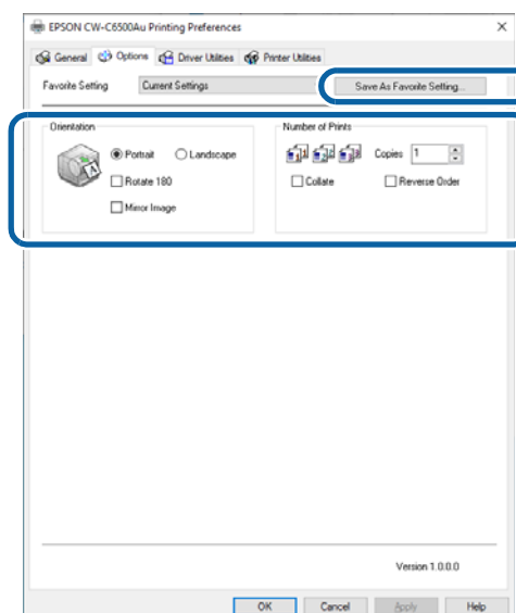
[Options] window
