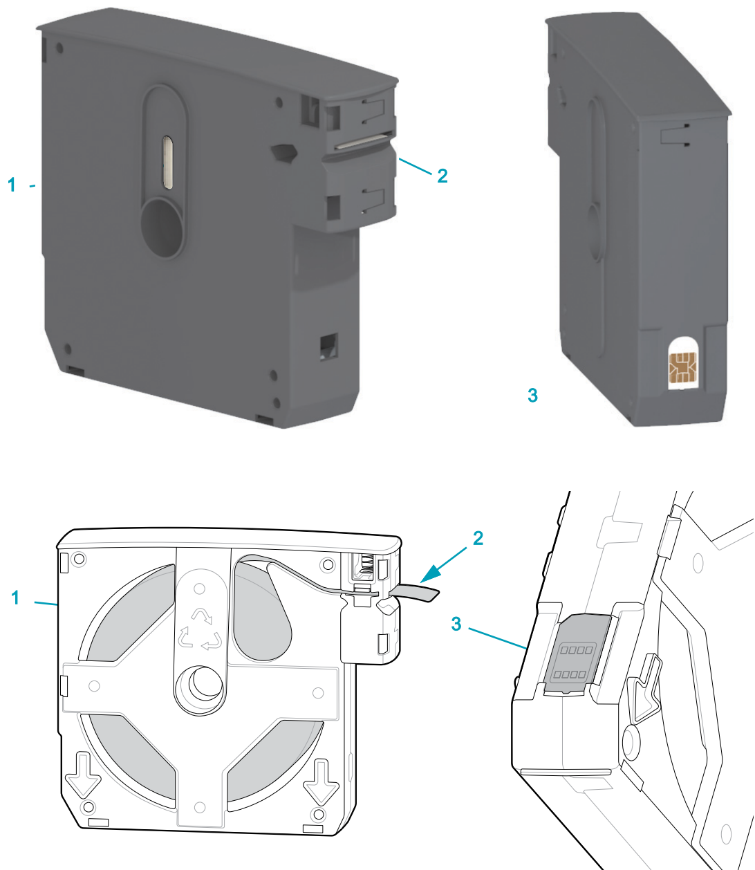
Figure 6 • Legacy Cartridge Features (Top) and Environmentally Friendly Cartridge Features (Bottom)
