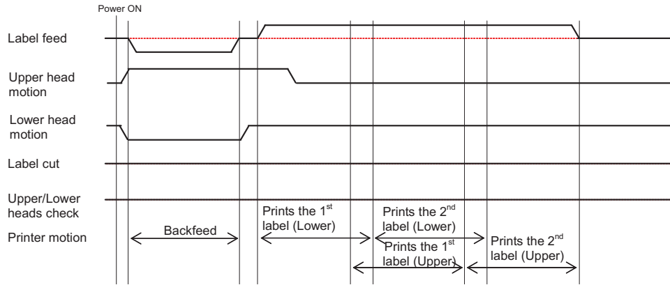
(2) Timing chart
