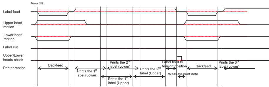
(2) Timing chart
