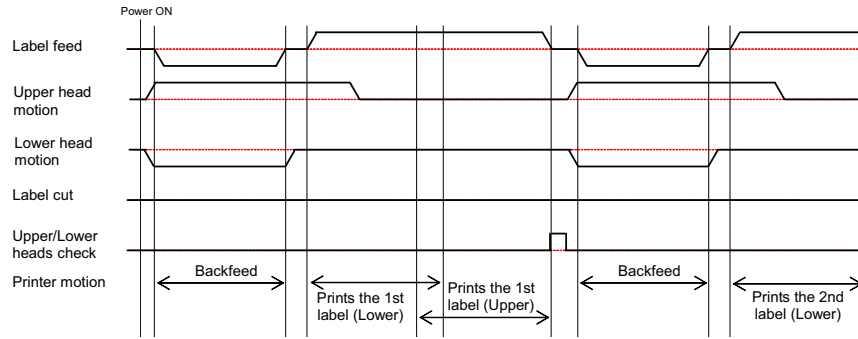
(2) Timing chart
