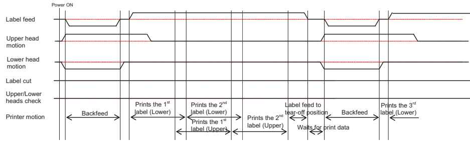
(2) Timing chart
