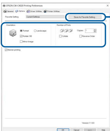
[Options] window
